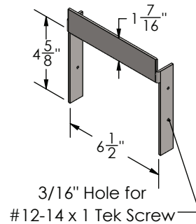
Part No. P-06C-DS
