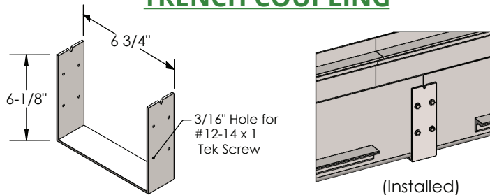
Part No. P-06UC
