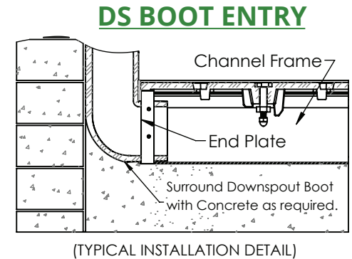
Part No. P-06C-DS
