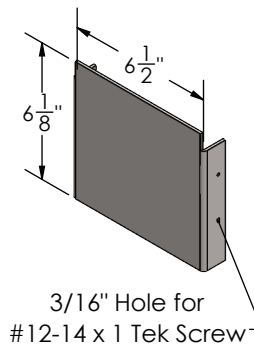
Part No. P-06C-CL
