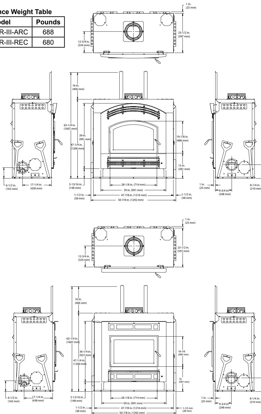
Figure 3.1 Appliance Dimensions
