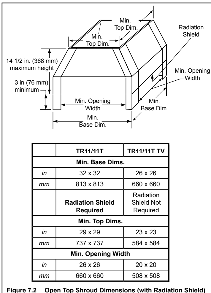
Figure 7.2 Open Top Shroud Dimensions (with Radiation Shield)
