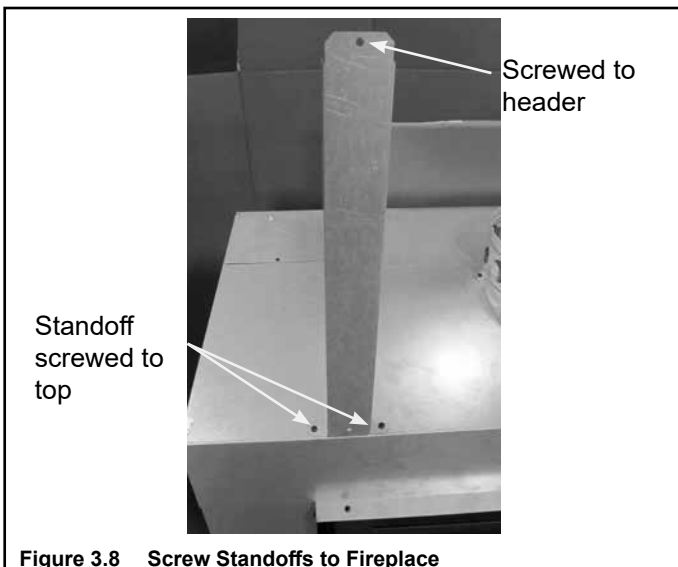
Figure 3.8 Screw Standoffs to Fireplace
