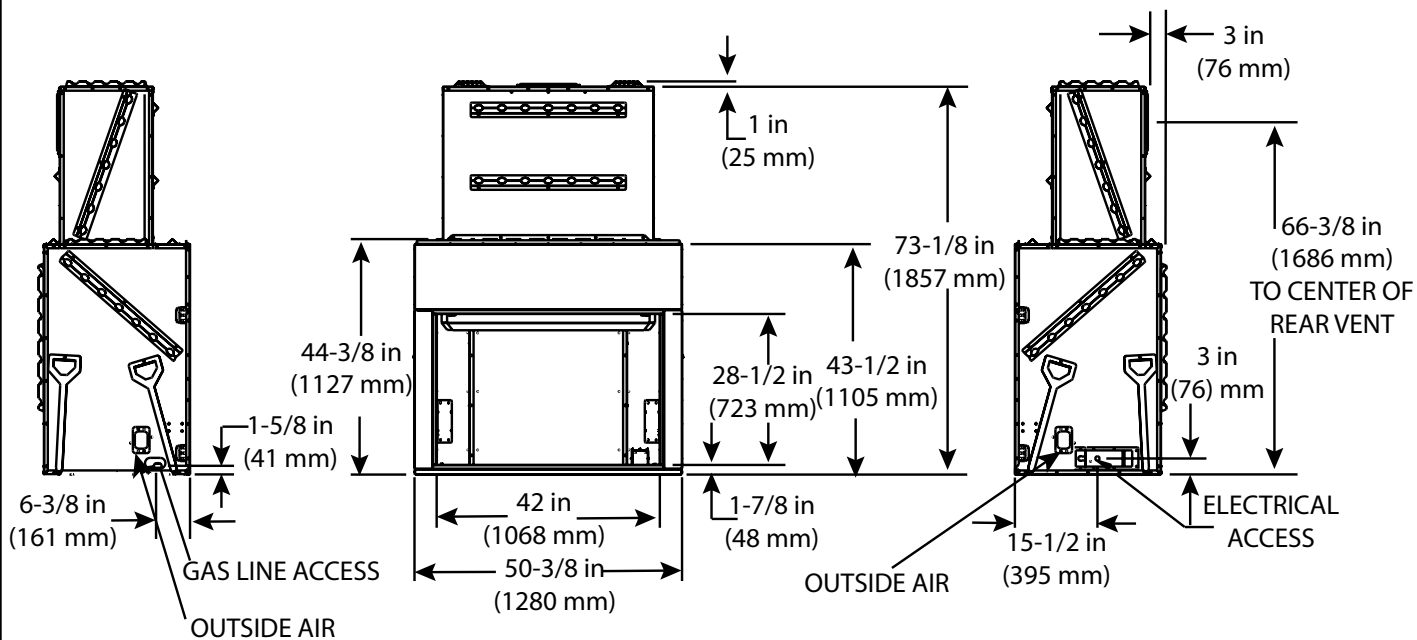
Figure 3.1 Appliance Dimensions
