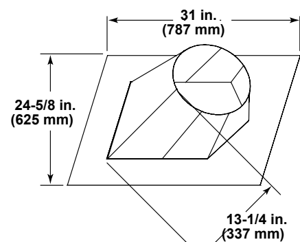
RF12 Roof Flashing
