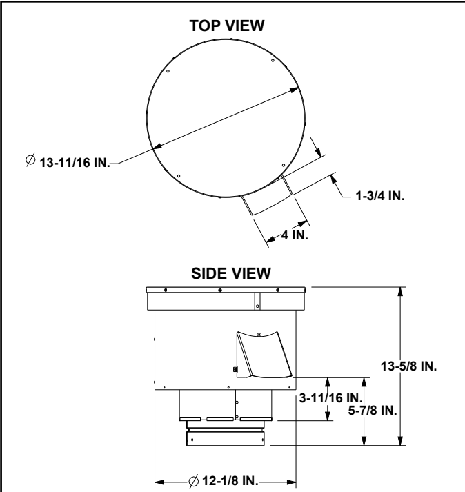
Figure 12.5 Vent Components
