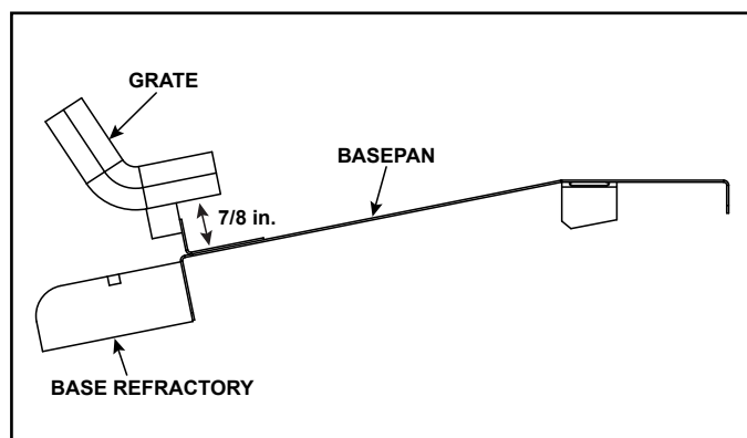
Figure 13. Side Profile Grate Location Reference
