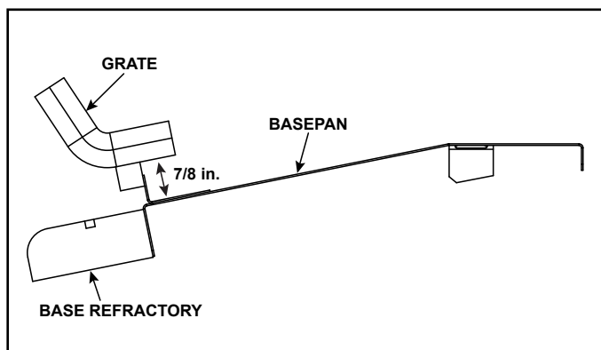
Figure 3. Side Profile Grate Location Reference
