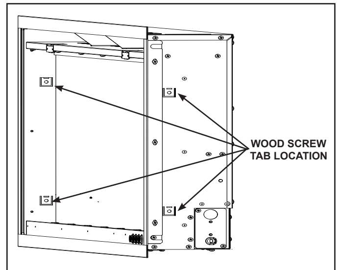
Figure 4.4 Securing the Appliance in 2 X 6 Framing
