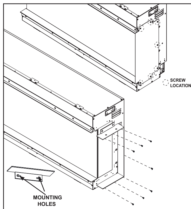
Figure 4.3 Plate Removal and Trim Install
