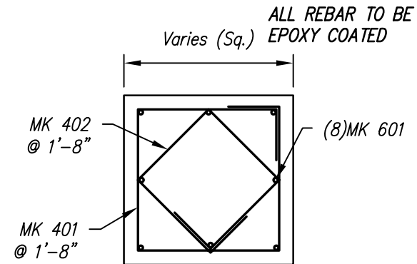
REINFORCING DETAIL
