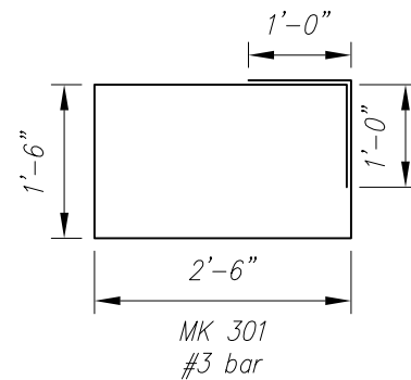
BENDING SCHEDULE
