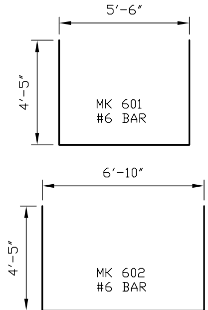
BENDING SCHEDULE
