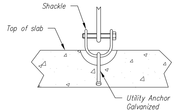
LIFTING DETAIL
