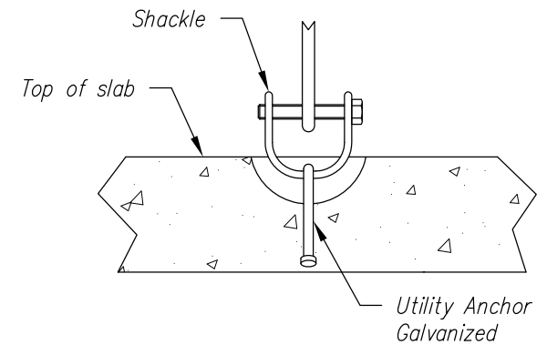
LIFTING DETAIL
