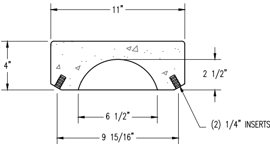
SECTION VIEW
