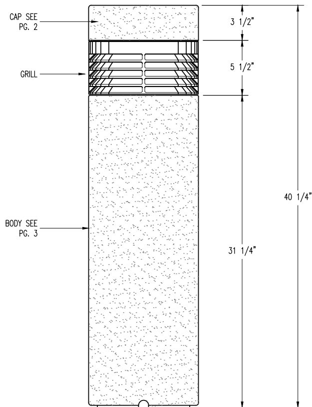
ELEVATION VIEW
