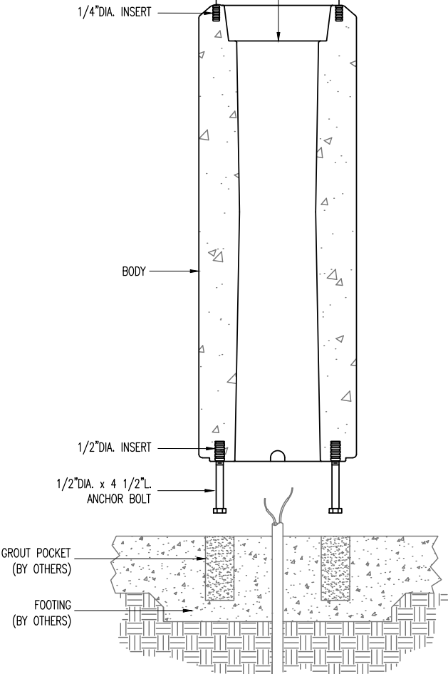
SECTION VIEW
