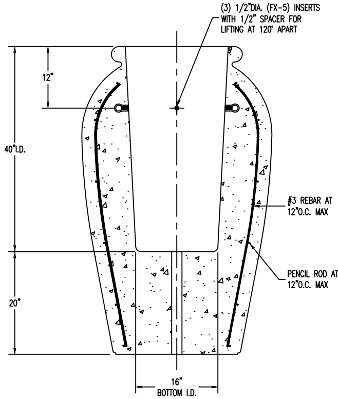
SECTION VIEW
