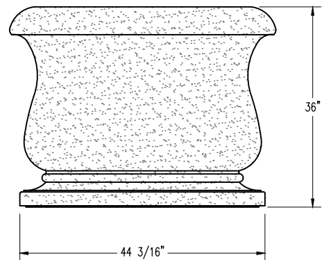
ELEVATION VIEW
