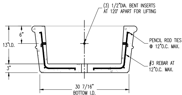
SECTION VIEW
