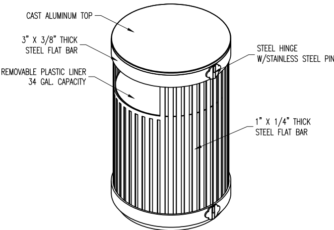
ISOMETRIC VIEW
