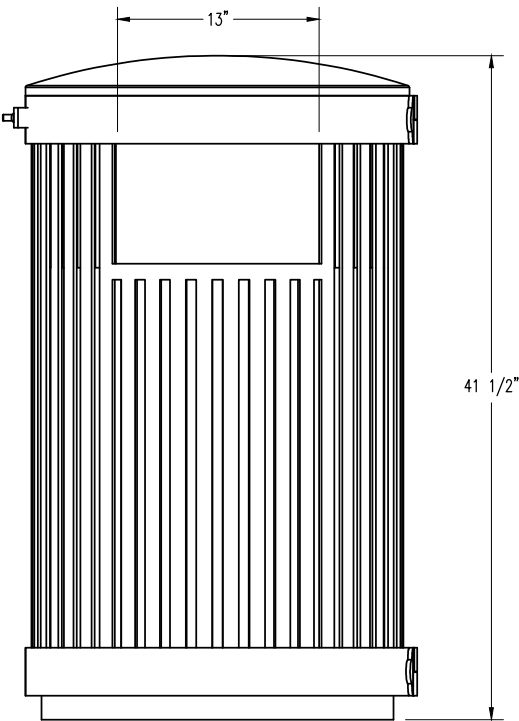
ELEVATION VIEW
