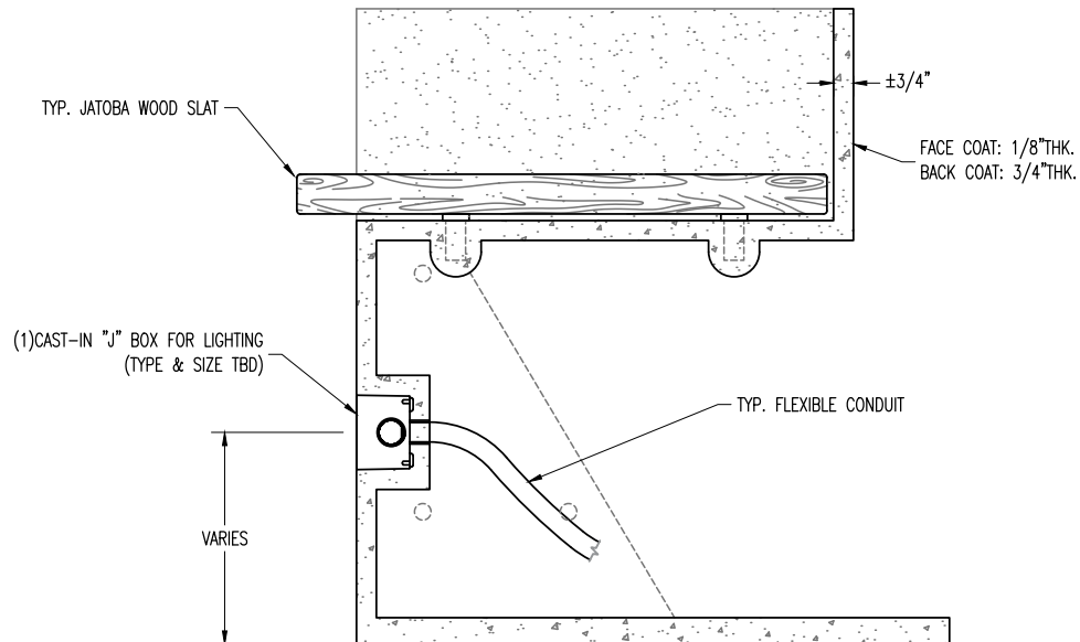
SECTION VIEW
