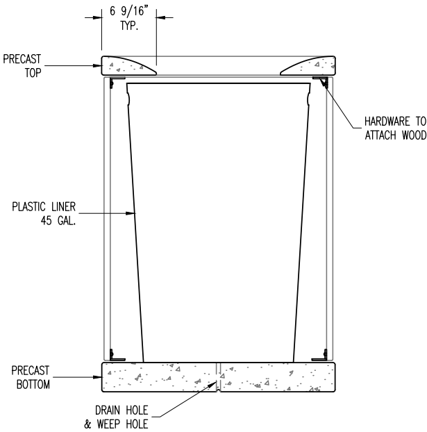
SECTION VIEW
