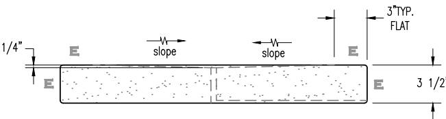
ELEVATION VIEW
