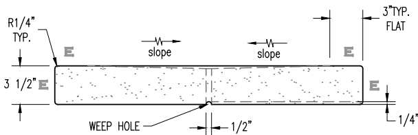
SIDE "A" VIEW
