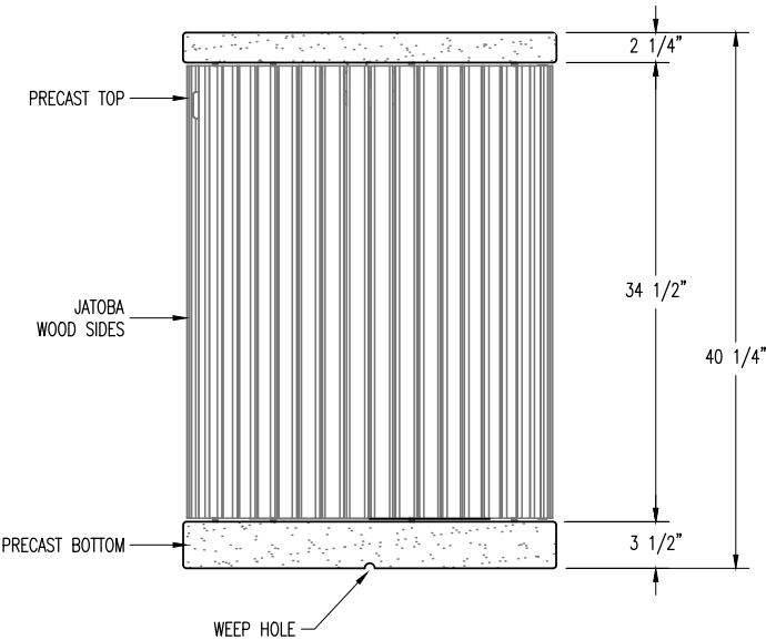
ELEVATION VIEW
