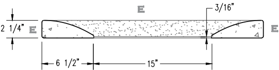
SECTION VIEW
