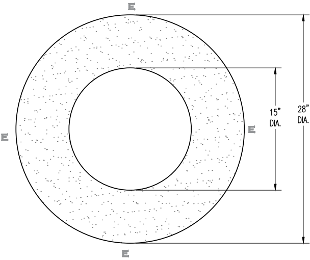
PLAN VIEW
