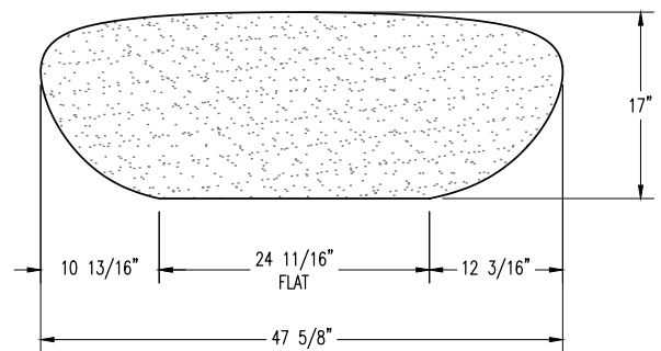
ELEVATION VIEW
