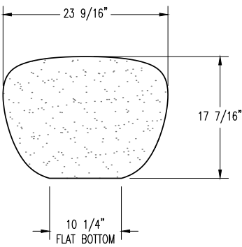
ELEVATION VIEW
