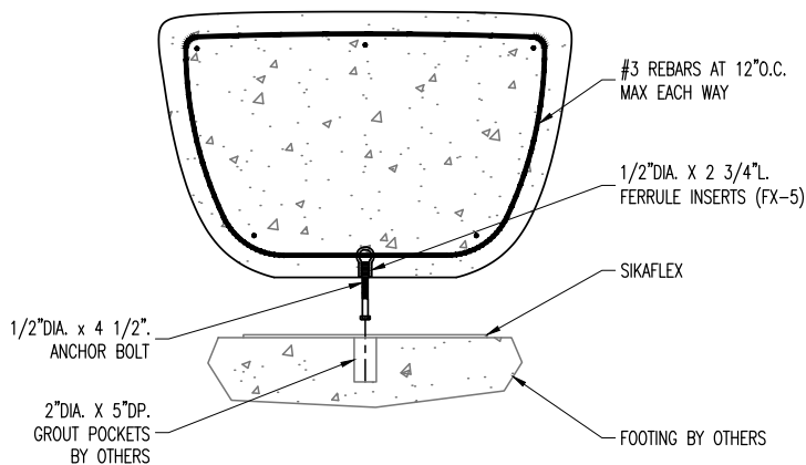
SECTION VIEW
