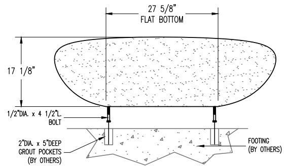
ELEVATION VIEW
