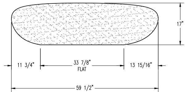
ELEVATION VIEW
