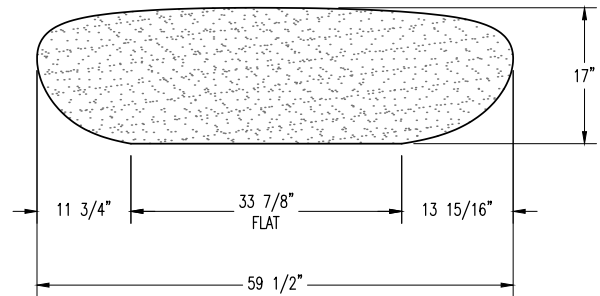
ELEVATION VIEW
