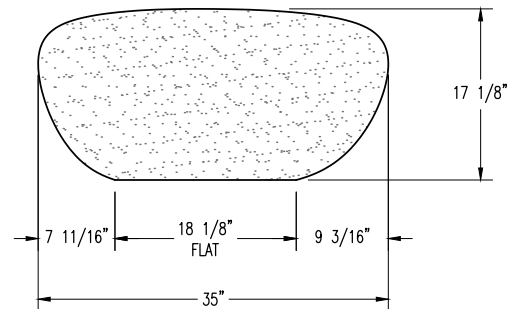
ELEVATION VIEW
