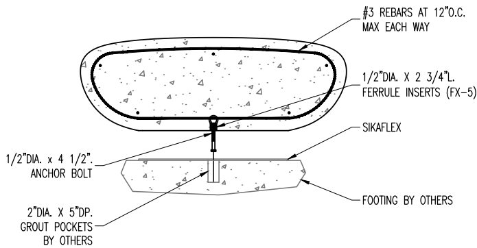
SECTION VIEW
