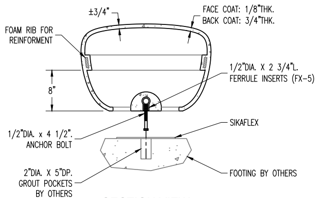
SECTION VIEW
