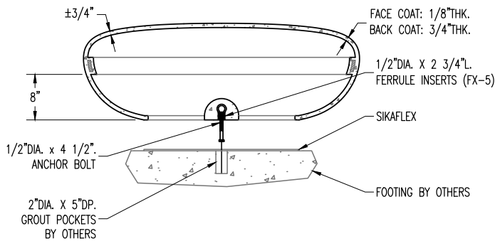
SECTION VIEW
