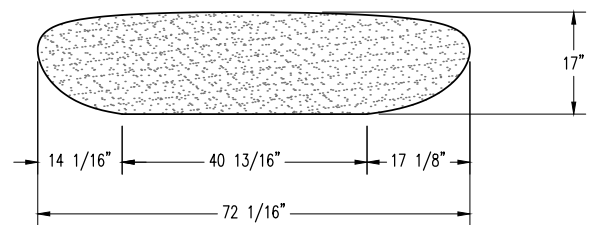
ELEVATION VIEW
