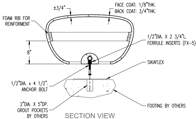
SECTION VIEW
