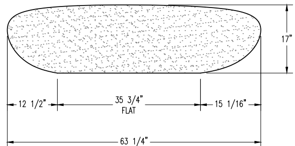
ELEVATION VIEW
