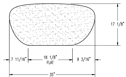
ELEVATION VIEW
