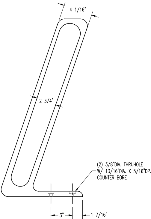
SECTION VIEW
