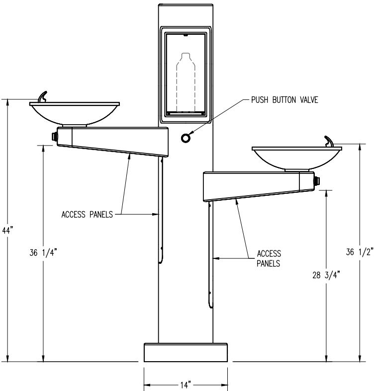
ELEVATION VIEW
