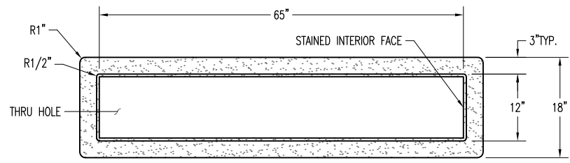
ELEVATION VIEW
