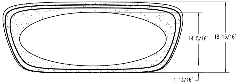
ELEVATION VIEW
