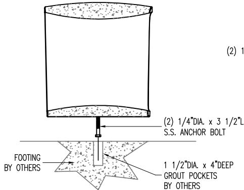
SECTION VIEW
