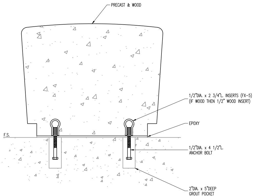
SECTION VIEW
