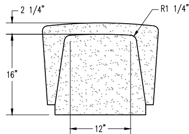
SIDE "A" VIEW
