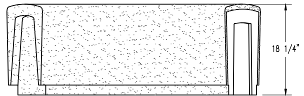
ELEVATION VIEW
