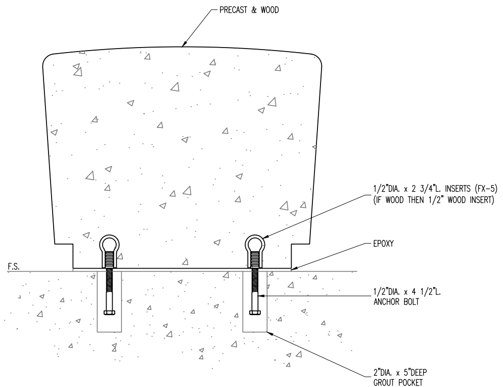
SECTION VIEW
