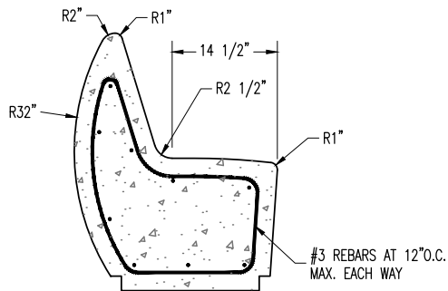
SECTION VIEW
