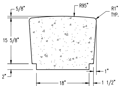
SECTION VIEW
