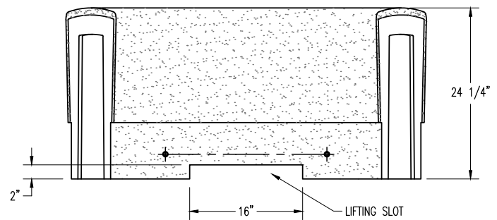
ELEVATION VIEW
