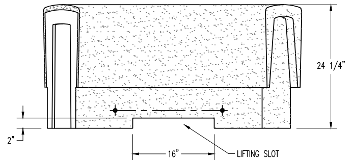
ELEVATION VIEW
