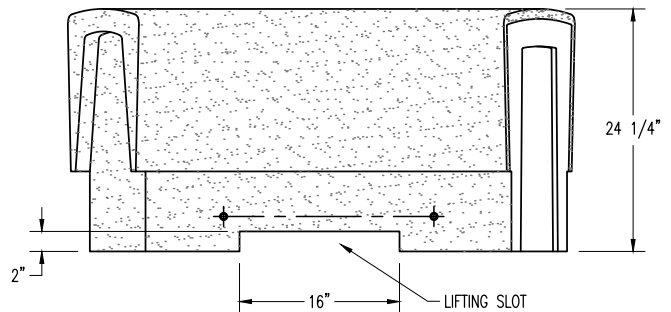
ELEVATION VIEW
