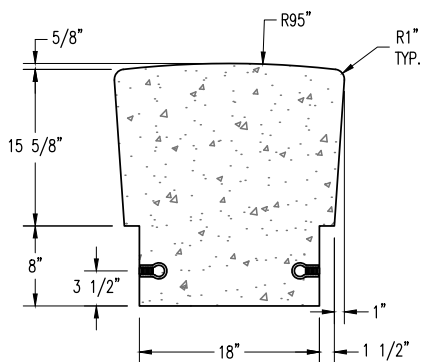
SECTION VIEW
