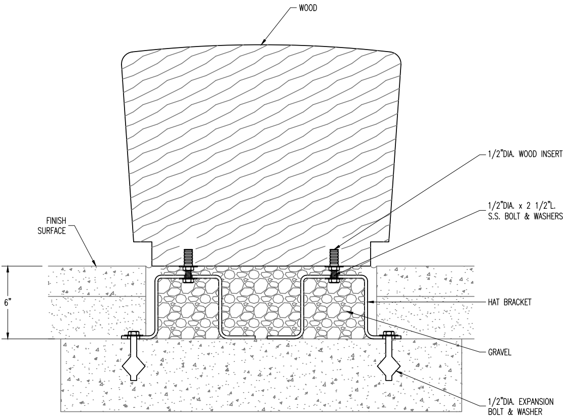
SECTION VIEW
