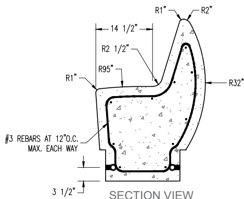
SECTION VIEW
