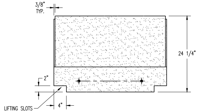
ELEVATION VIEW
