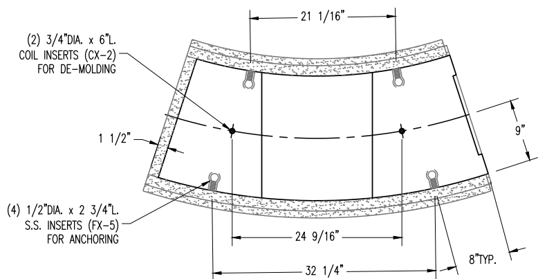
BOTTOM VIEW
