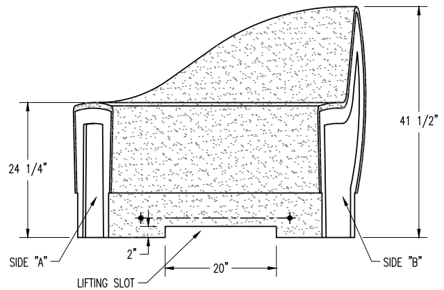
ELEVATION VIEW
