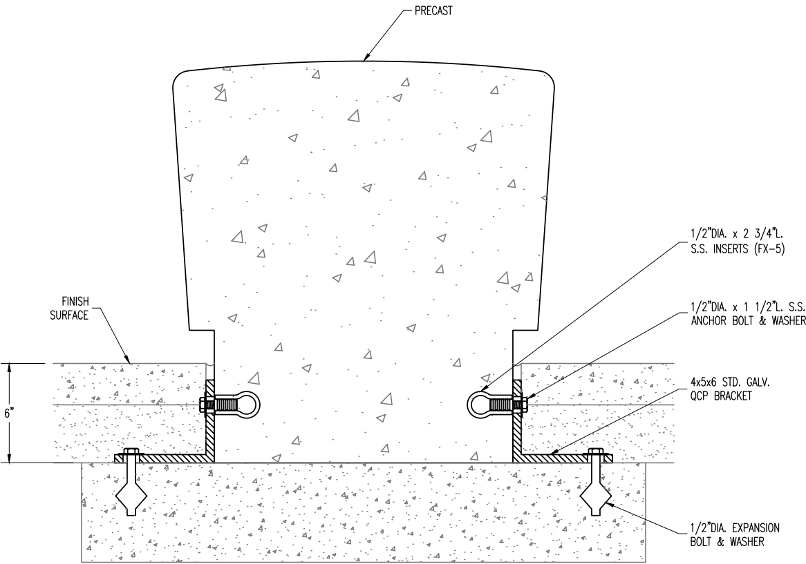
SECTION VIEW
