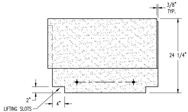
ELEVATION VIEW
