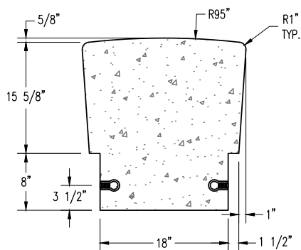
SECTION VIEW
