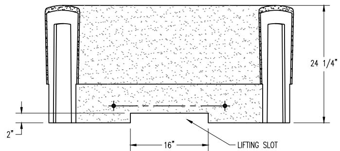
ELEVATION VIEW
