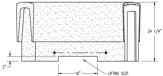
ELEVATION VIEW
