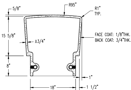
SECTION VIEW
