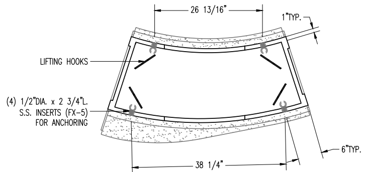
BOTTOM VIEW
