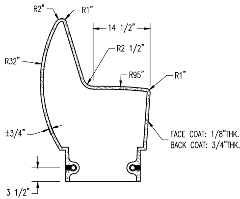
SECTION VIEW
