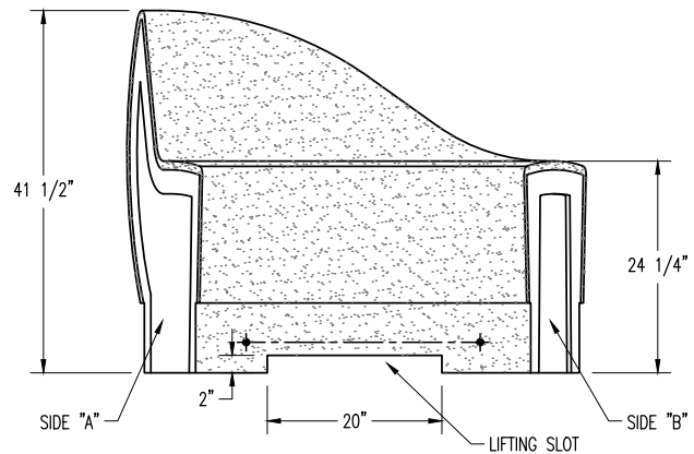
ELEVATION VIEW
