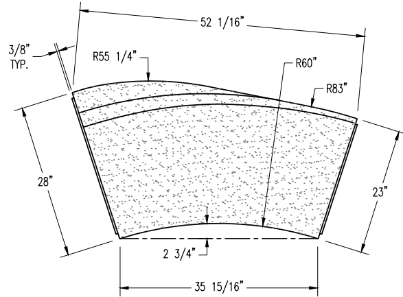
PLAN VIEW
