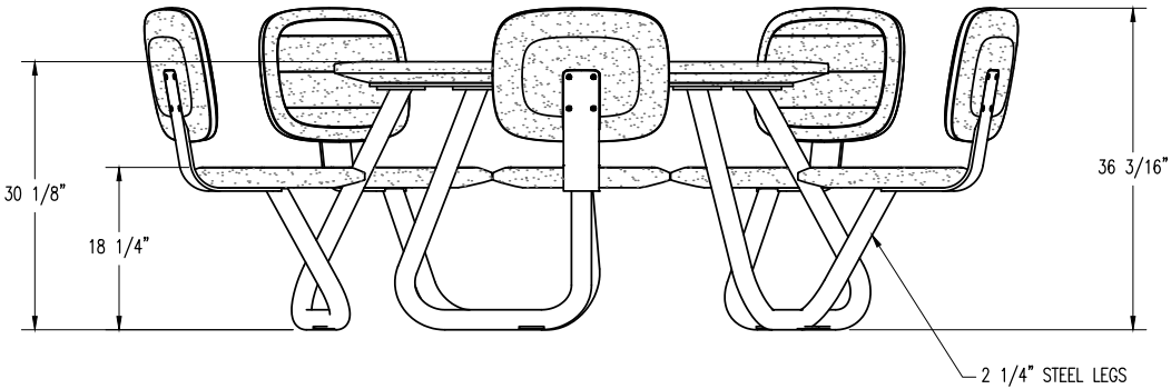
ELEVATION VIEW
