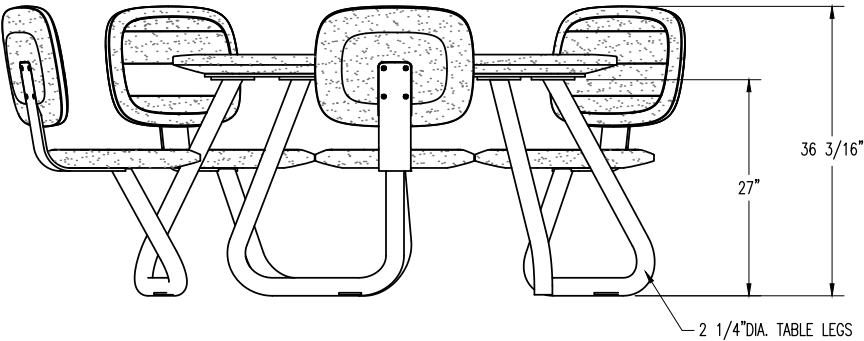
ELEVATION VIEW
