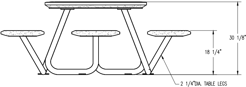
ELEVATION VIEW
