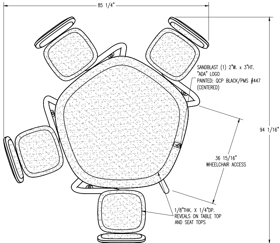
PLAN VIEW
