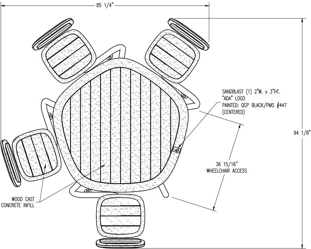
PLAN VIEW
