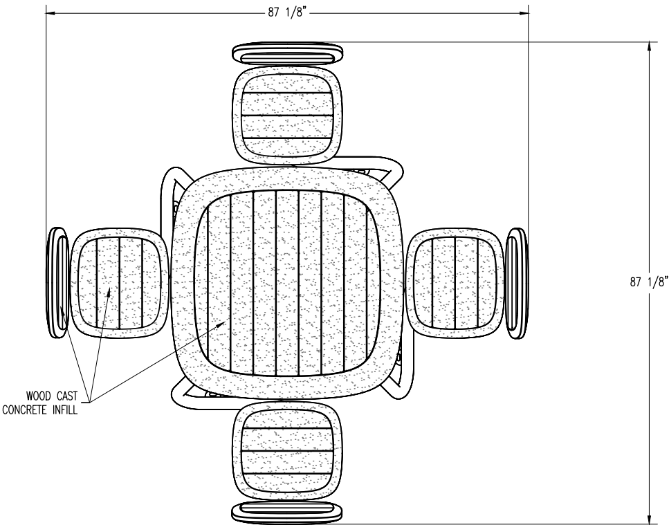
PLAN VIEW
