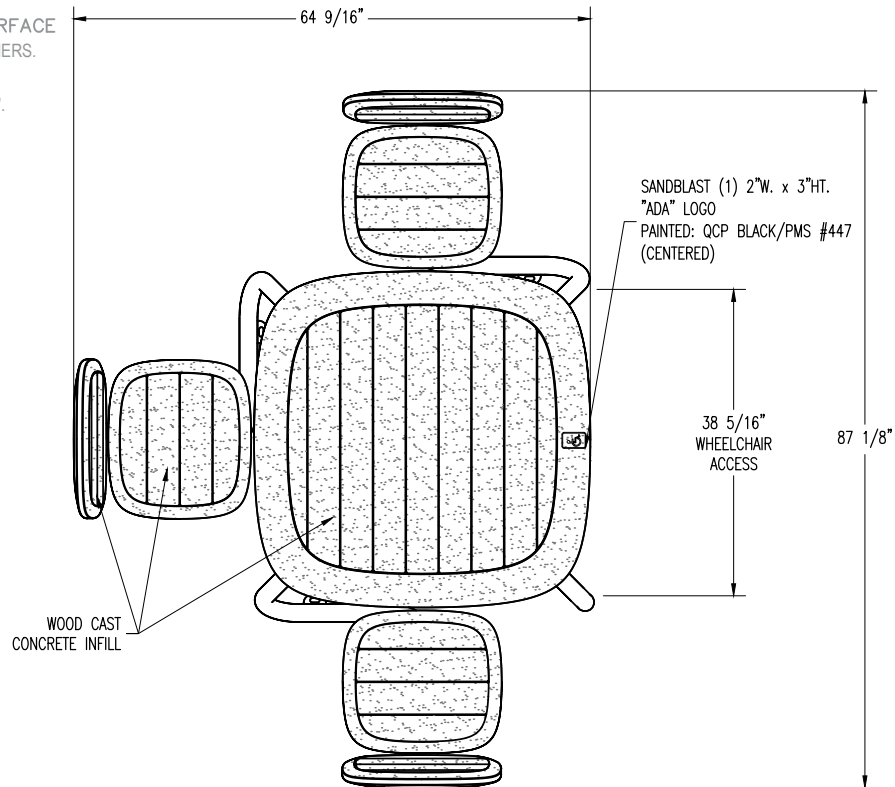
PLAN VIEW
