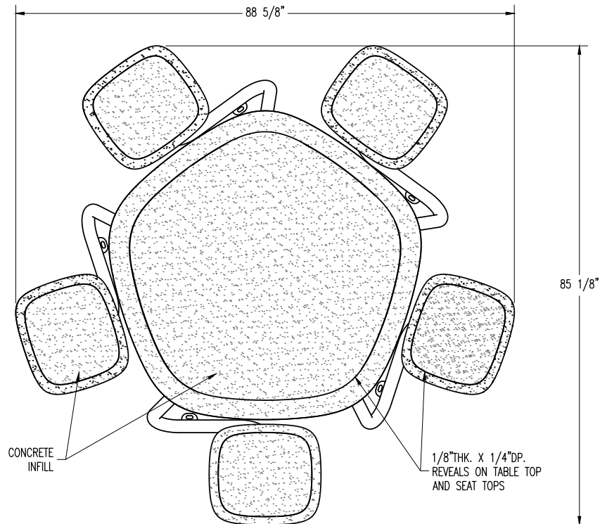
PLAN VIEW
