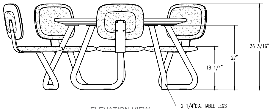
ELEVATION VIEW
