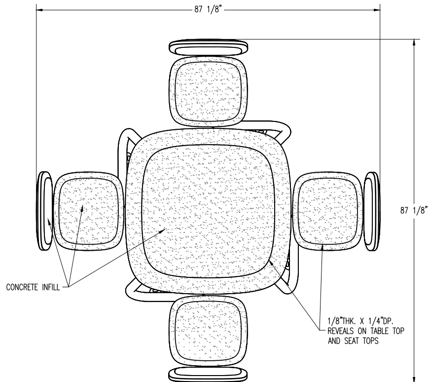
PLAN VIEW
