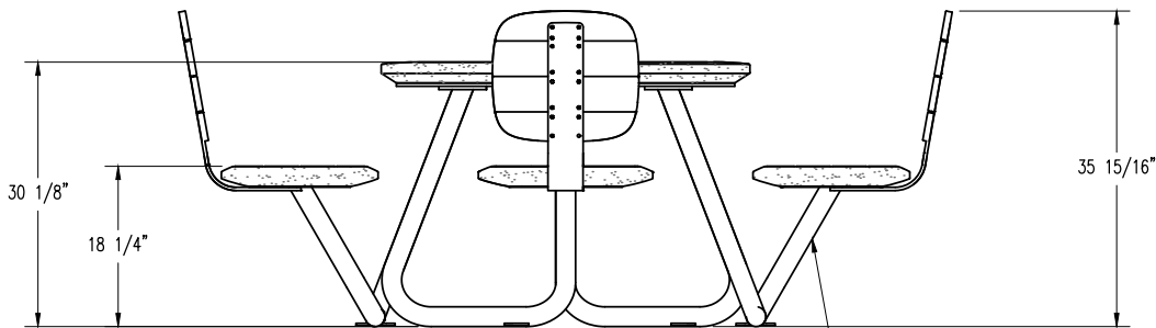
ELEVATION VIEW
