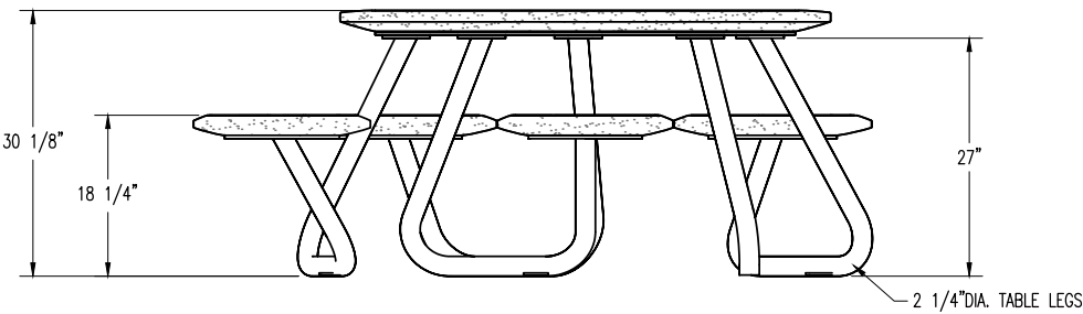
ELEVATION VIEW
