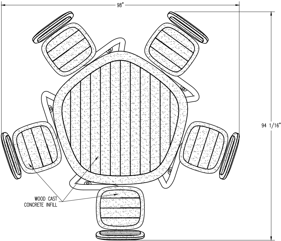
PLAN VIEW
