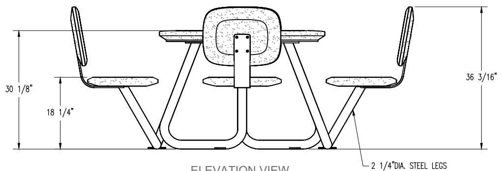
ELEVATION VIEW
