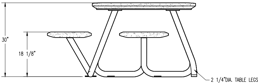
ELEVATION VIEW
