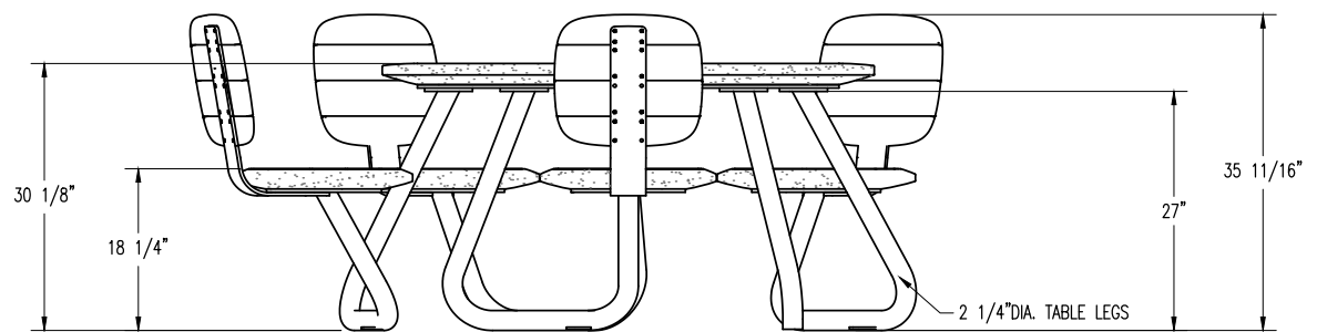
ELEVATION VIEW
