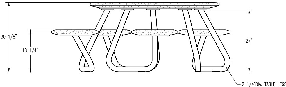
ELEVATION VIEW
