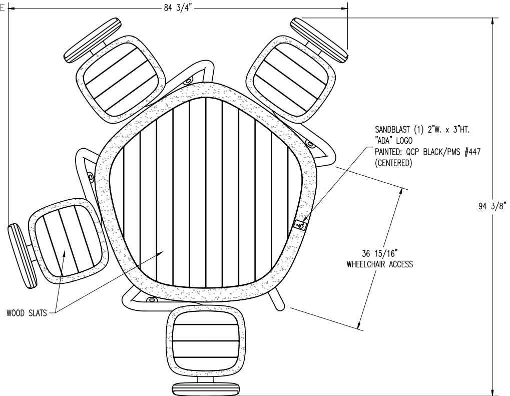
PLAN VIEW
