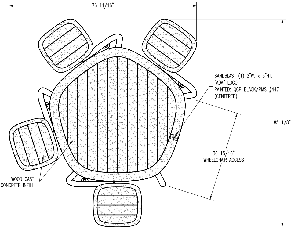
PLAN VIEW
