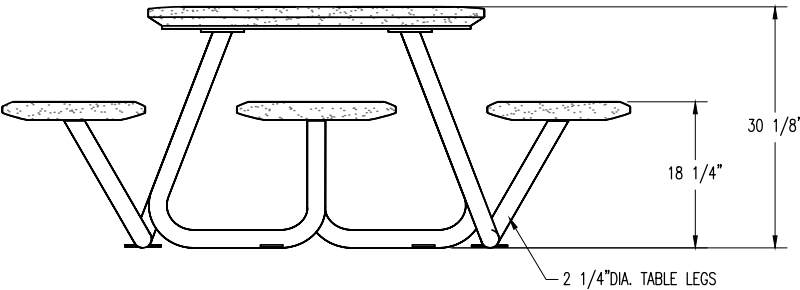
ELEVATION VIEW
