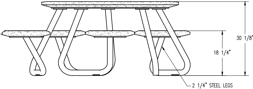
ELEVATION VIEW
