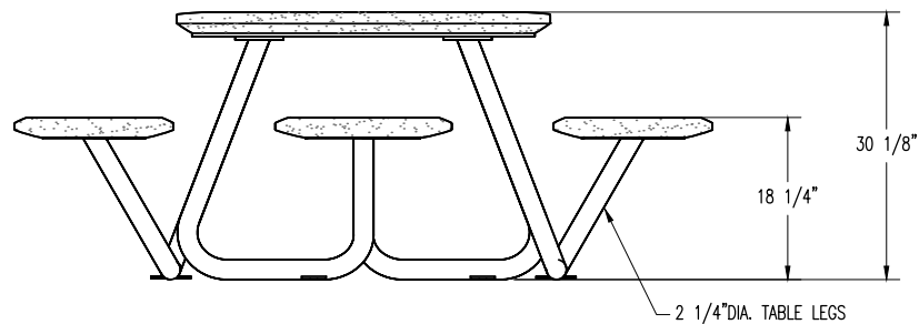
ELEVATION VIEW
