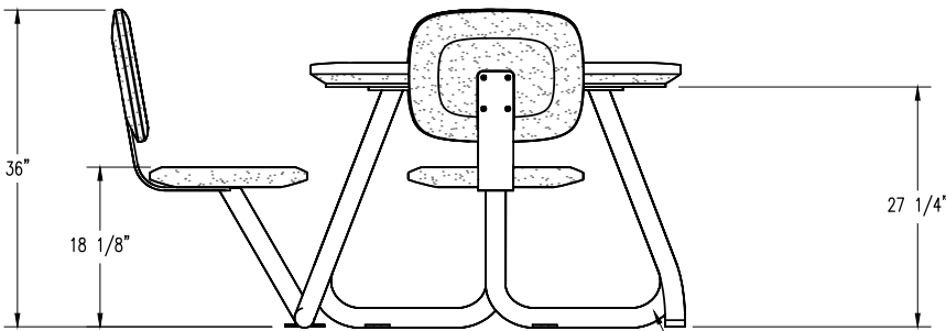
ELEVATION VIEW
