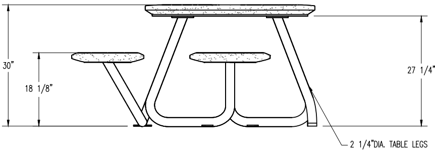
ELEVATION VIEW
