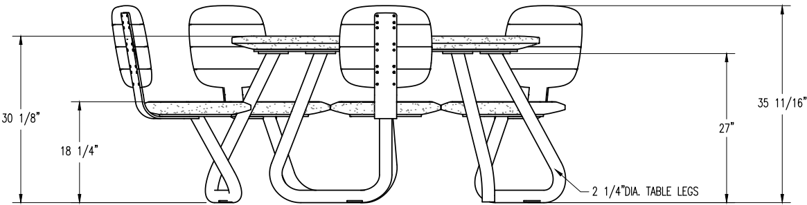
ELEVATION VIEW
