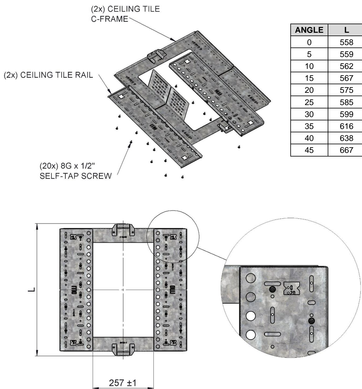
Fig 4 – Sloped Ceiling - Angles
