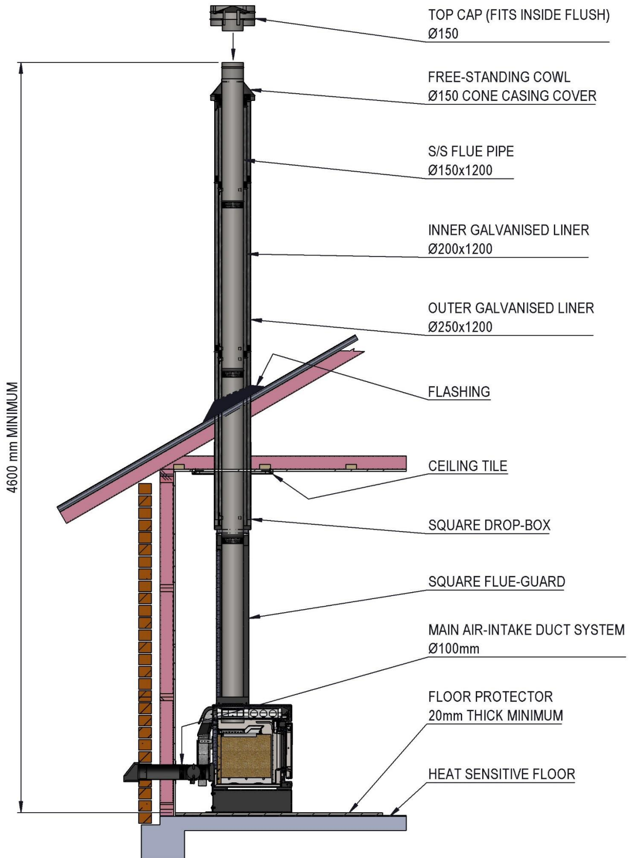
FIG. C: OLLI FREESTANDING WOODBURNER - TYPICAL FLUE INSTALLATION
