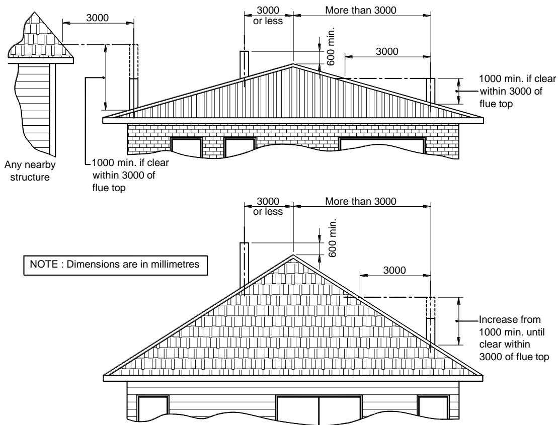
FIG D: FLUE SYSTEM REQUIREMENTS (Not to scale)
