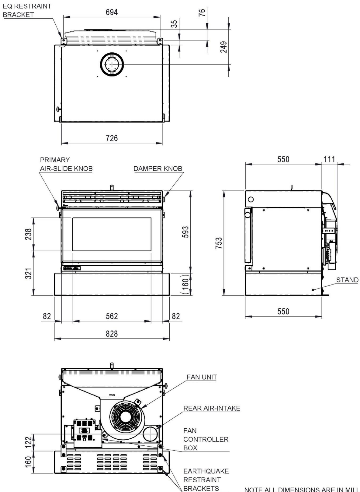
FIG. A: HEATER DIMENSIONS – OLLI WOODBURNER (Not to Scale.)
