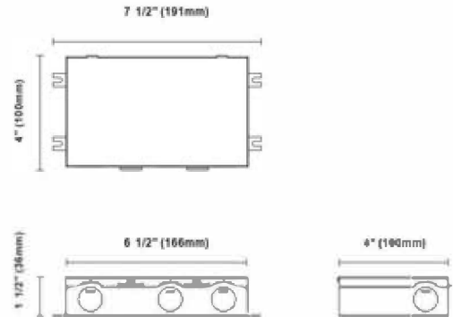
KIG-020-WDJ Triac/0-10V/1-10V LED DRIVER 10w/15w/17w/18w/20w 120-277V [250mA, 350mA, 400mA, 450mA, 500mA, 600mA, 700mA]
