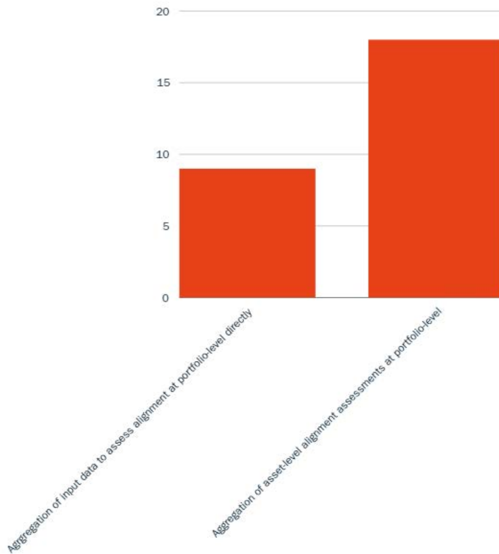
Figure 37: Count of methodologies reviewed per aggregation approach.
