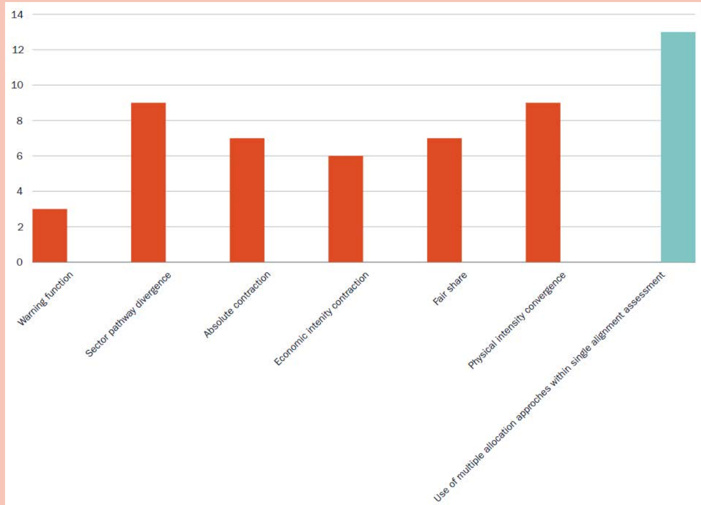
Figure 35: Count of methodologies reviewed using the following allocation approaches
