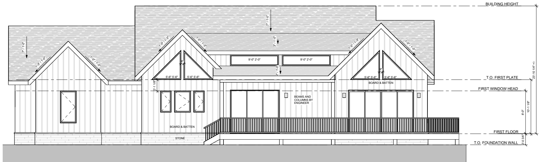
2 REAR VIEW
