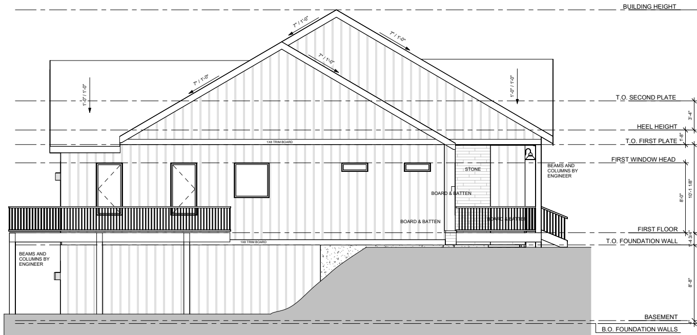
1LEFT VIEW
