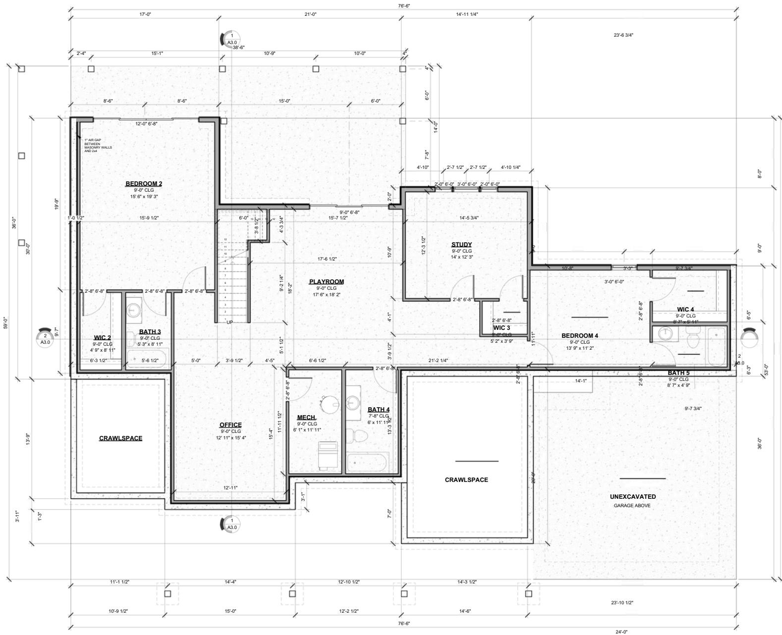
1BASEMENT FOUNDATION PLAN
