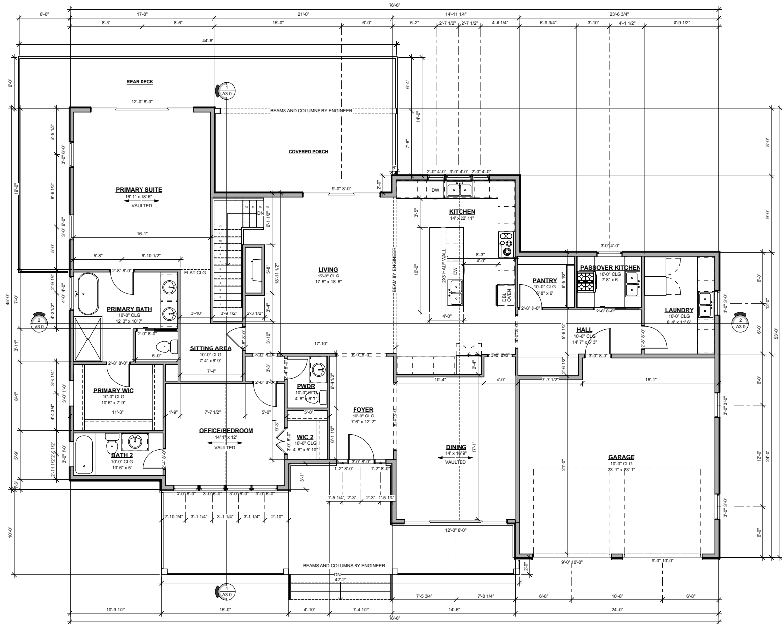
1FIRST FLOOR PLAN
