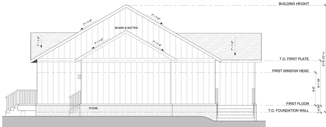
1 RIGHT VIEW 1/4" = 1'-0"
