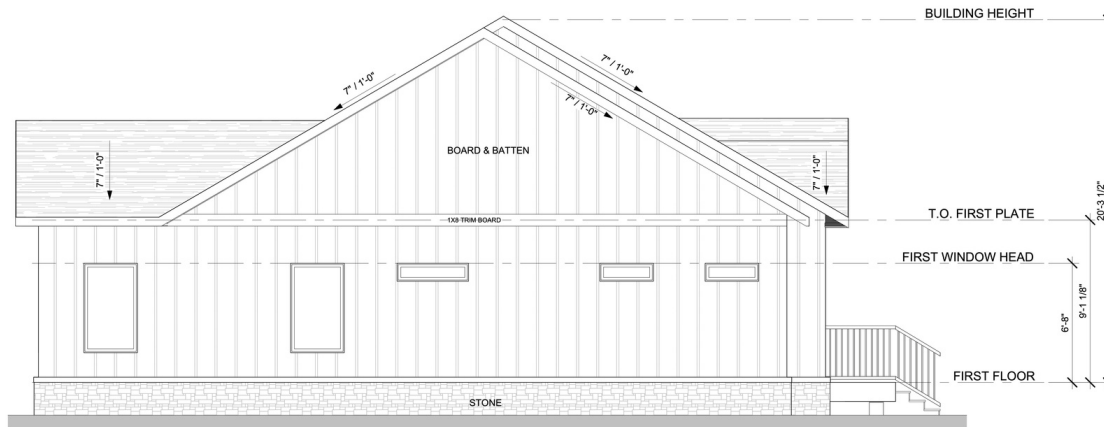
1 LEFT VIEW 1/4" = 1'-0"
