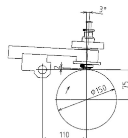
Positional relationship between drum and test piece
