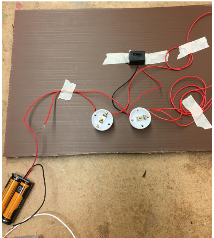
Back of the question board: wires from the brass pins connected to the light bulbs, buzzer, and battery pack.
