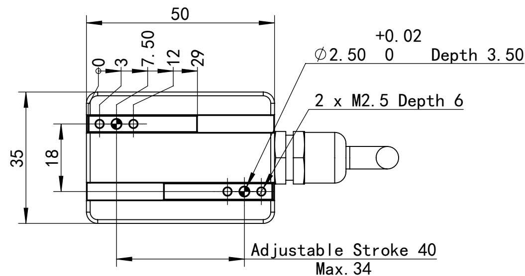
A-Direction View
