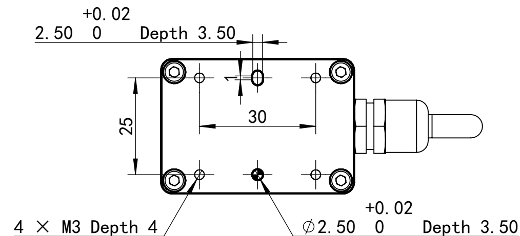
B-Direction View
