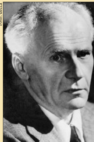
Wilhelm Backhaus
