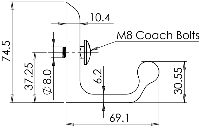
DETAIL A SCALE 1 : 1.75 Extrusion Profile and Bolt
