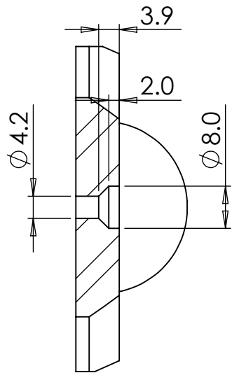
SECTION A-A 2 Positions
