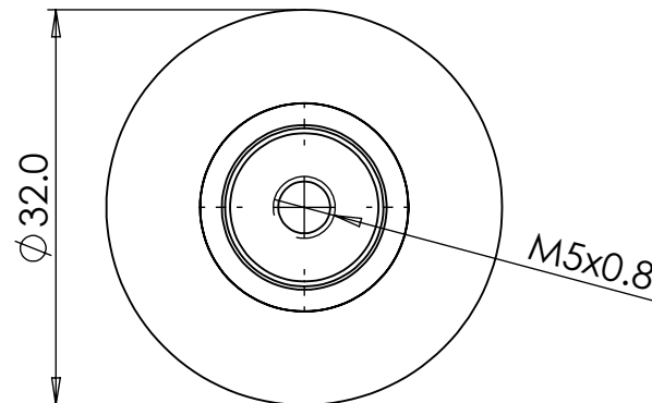
Medium Art Deco Knob: Ø 32 mm, Projection 33 mm
