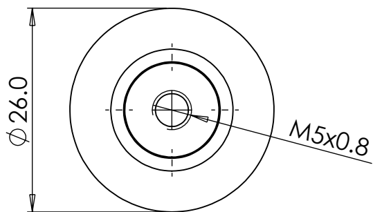
Small Art Deco Knob: Ø 26 mm, Projection 30 mm
