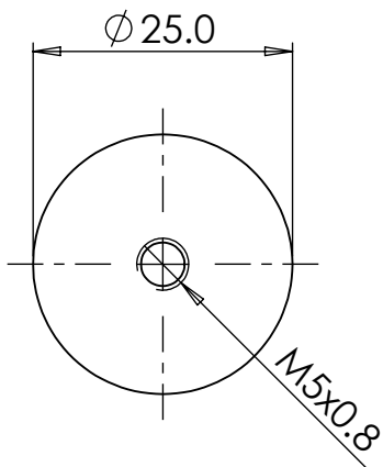
Small Beehive Knob
