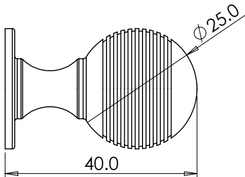
Small Beehive Knob
