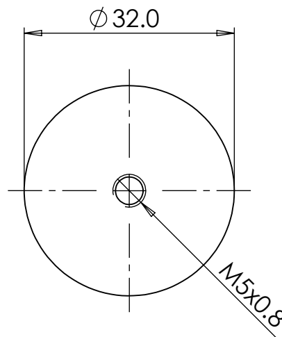
Large Beehive Knob
