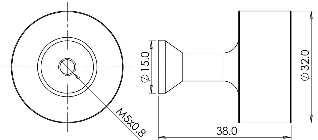
Large Circle Art Deco Cupboard Knob: Ø 32 mm, Projection 38 mm (Base Ø 15 mm)
