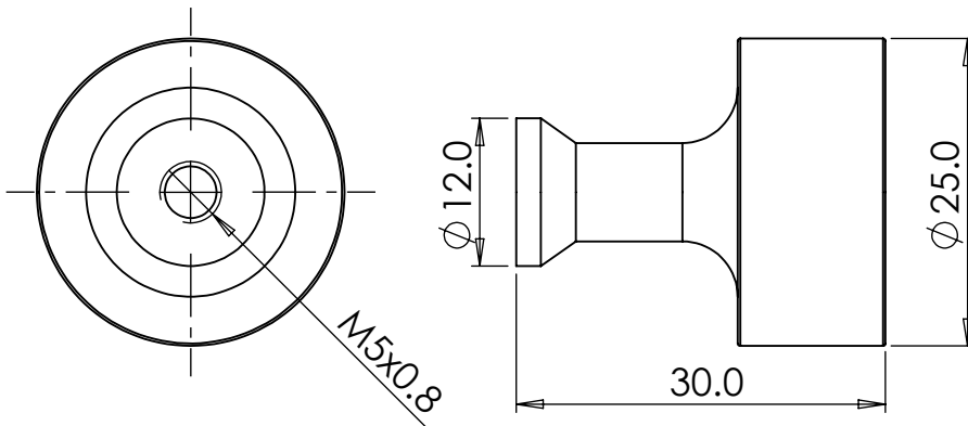
Medium Circle Art Deco Cupboard Knob: Ø 25 mm, Projection 30 mm (Base Ø 12 mm)
