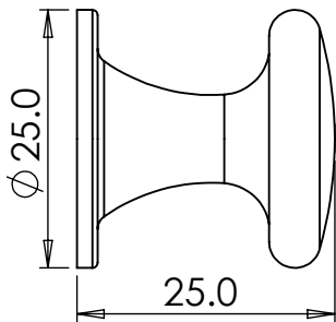
Small Cushion Knob: Ø 25 mm, Projection 25 mm
