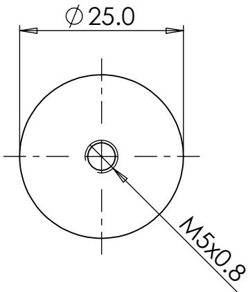
Small Cushion Knob: Ø 25 mm, Projection 25 mm
