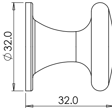
Medium Cushion Knob: Ø 32 mm, Projection 32 mm
