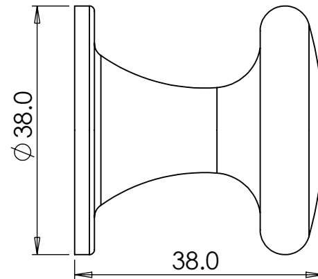
Large Cushion Knob: Ø 38 mm, Projection 38 mm
