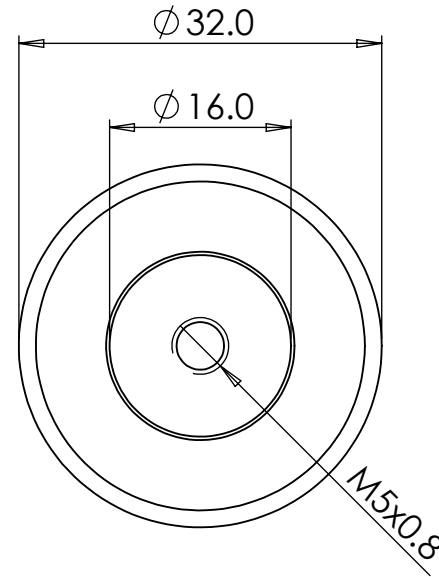
Large Grooved Art Deco Knob: \varnothing 32 mm, Projection 32 mm (Base \varnothing 16 mm)
