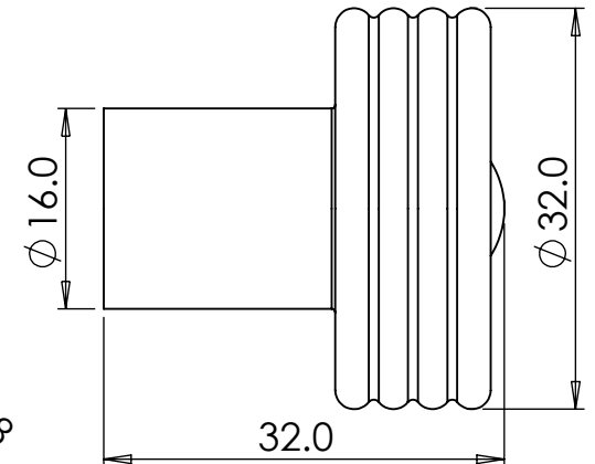
Large Grooved Art Deco Knob: \varnothing 32 mm, Projection 32 mm (Base \varnothing 16 mm)
